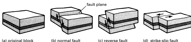
Types of fault
