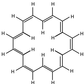
[18]-annulene
