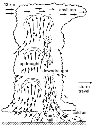
Cross section through a thunderstorm cell
