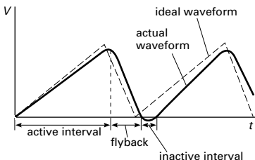
Sawtooth waveform
