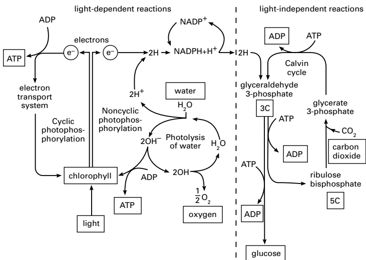
Photosynthesis
