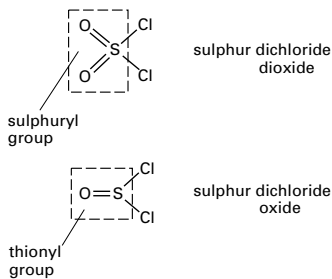
Oxychlorides of sulphur
