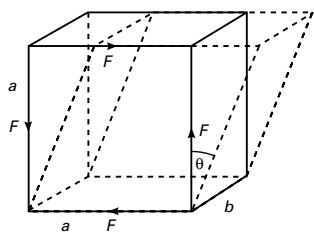
Shearing force
