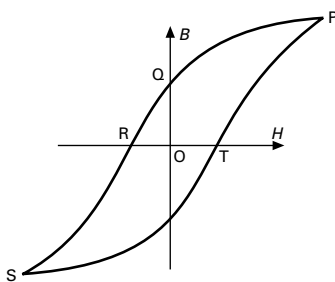
Hysteresis
