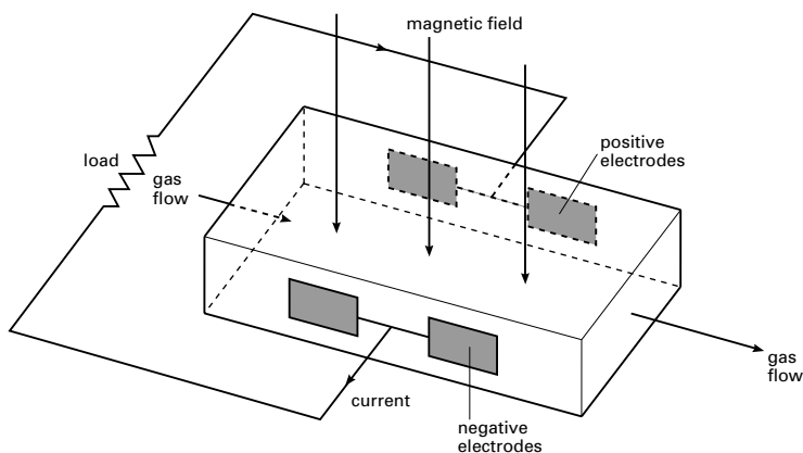
Magnetohydrodynamic generator
