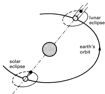
Solar and lunar eclipses
