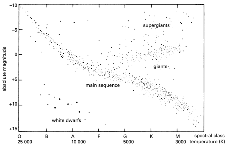
Hertzsprung–Russell diagram
