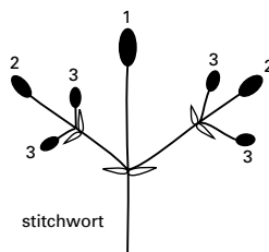
dichasial cyme
