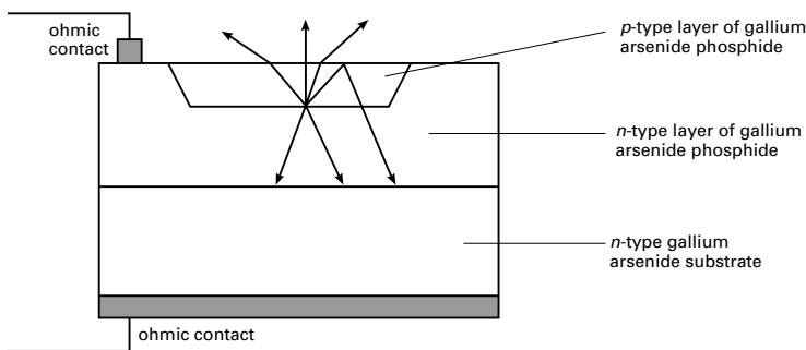
Light-emitting diode
