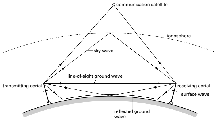
Radio transmission
