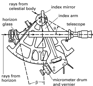
A sextant
