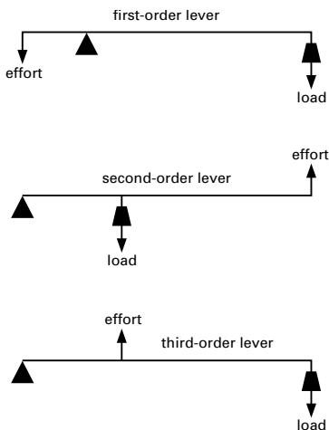
Levers
