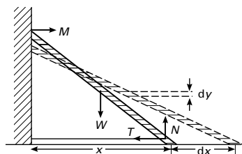
Virtual work
