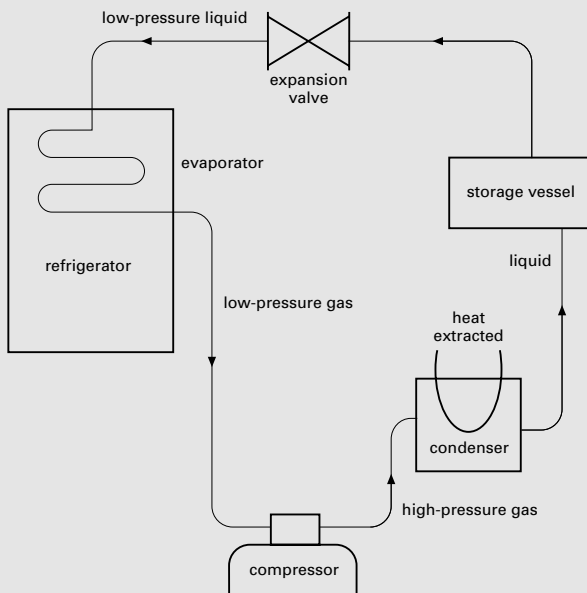
Vapour-compression cycle
